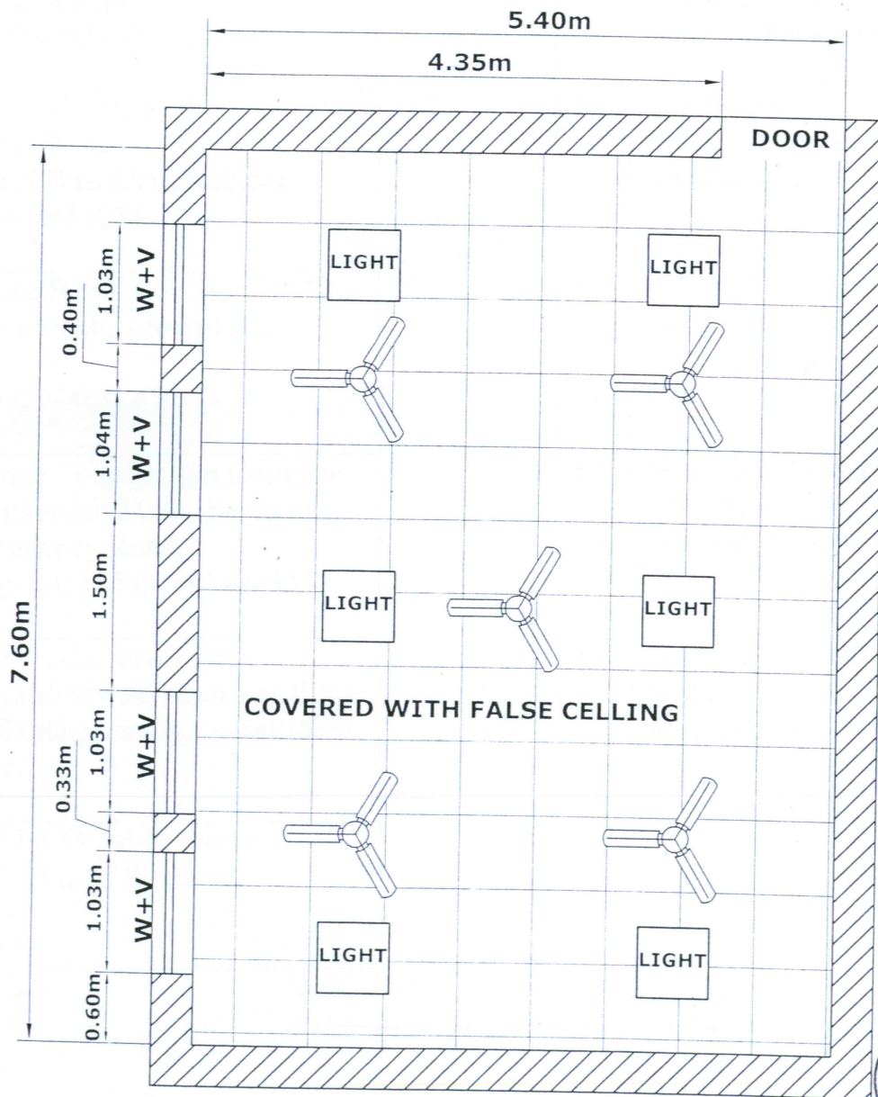
Layout plan of Repair and Renovation of Lab (False ceiling including LED Lights & Aluminium work for covering of windows and ventilators of Biotechnology lab) at Div.-III, ICAR- CAZRI, Jodhpur
